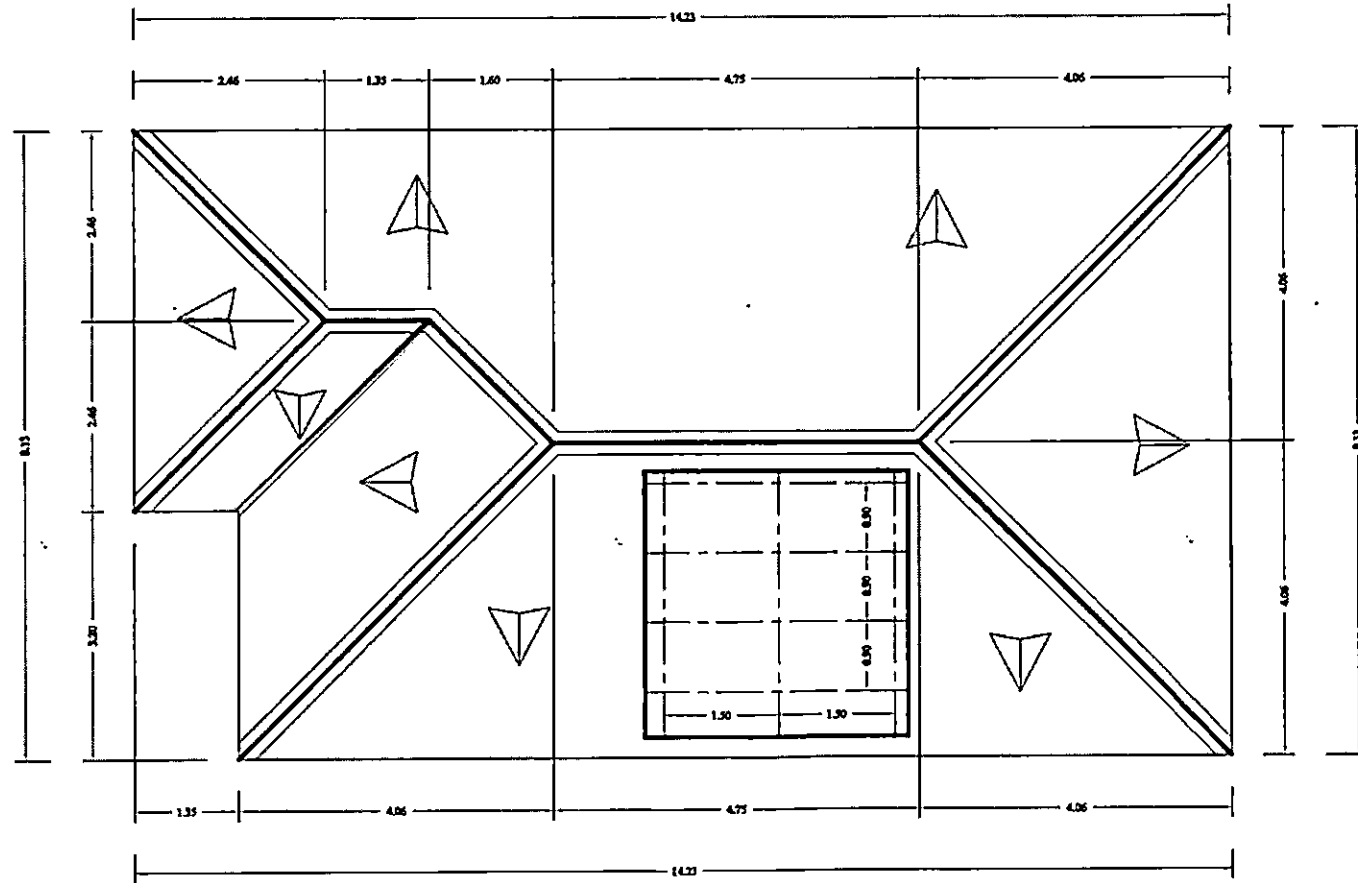
ROOF PLAN
