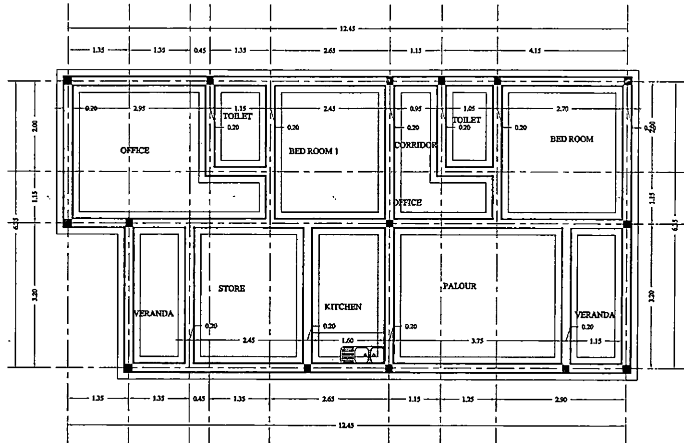
FOUNDATION PLAN
