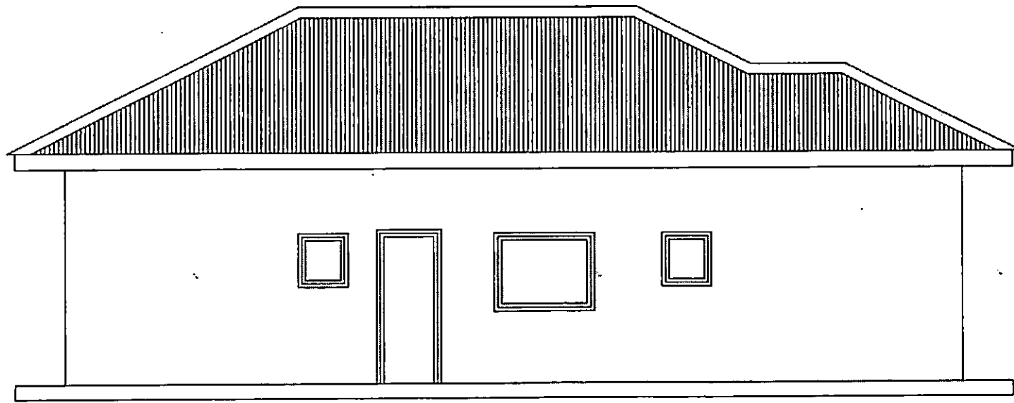
BACK VIEW
